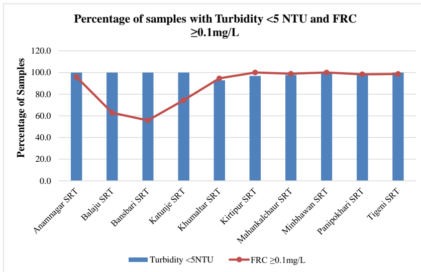
Graph showing the percentage of samples with Turbidity and FRC within NDWQS limit
