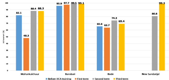
Percentage of samples achieving turbidity of 5 NTU or less
