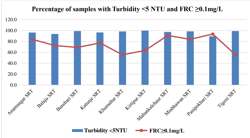
Graph showing percentage of samples with Turbidity and FRC within NDWQS limit
